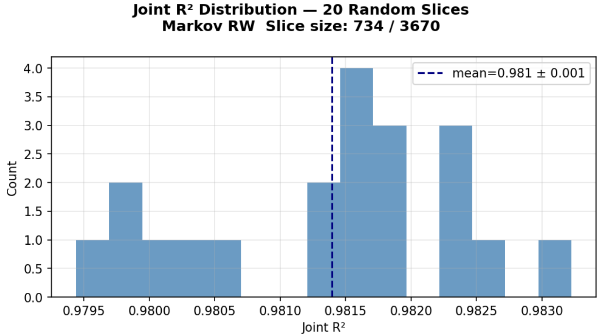
Figure 8: Distribution of Joint R^2 across 20 random slices, nearest-neighbor random walk. All 20 draws fall in the range 0.979–0.984 with \text{std} = 0.001 . The continuously varying asymmetry q across 5,000 distinct environments is linearly readable from any same-size window into the converged parameter vector, with no discreteness artifact inflating the result.
