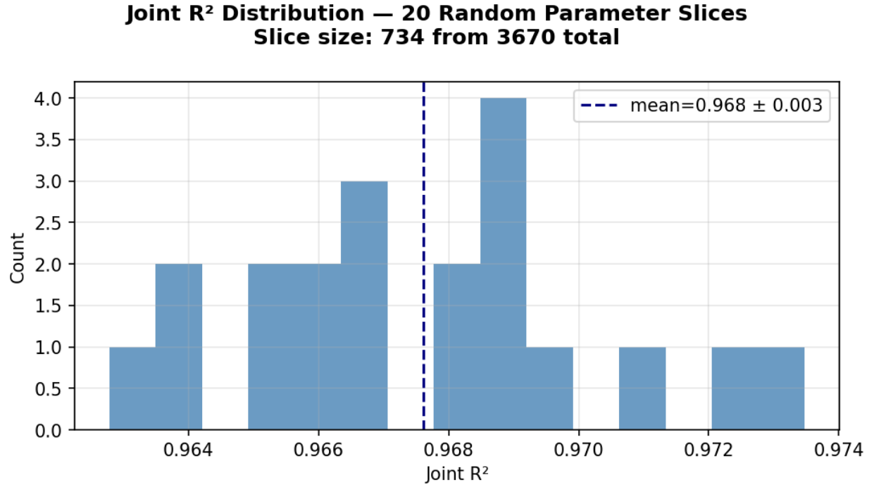
Figure 2: Distribution of Joint R^2 across 20 random parameter slices, quasi-periodic experiment. Each bar corresponds to one random draw of d = 734 parameters from the full D = 3,670 -dimensional parameter vector. The distribution is tightly concentrated (range 0.963–0.974, std = 0.003), confirming that Koopman spectral structure is recoverable from any same-size window into the parameter vector.
