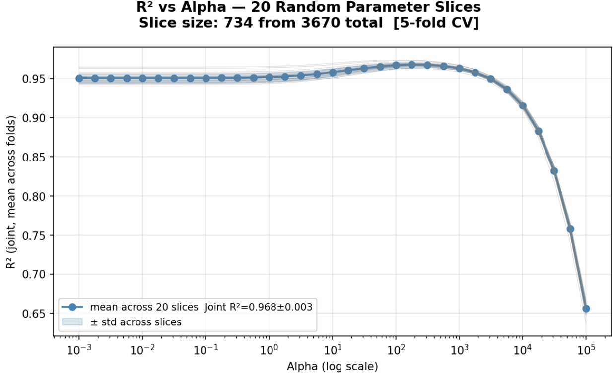
Figure 1: R^2 vs. \alpha curves, quasi-periodic experiment. Mean Joint R^2 \pm std across 5 folds as a function of regularization strength \alpha , for each of P = 20 independently drawn random parameter slices (grey curves) and their mean (blue). The curves are nearly indistinguishable throughout the plateau region, confirming that linear decodability of the Koopman spectrum is uniformly distributed across the parameter vector. Peak mean Joint R^2 = 0.968 \pm 0.003 . N = 5,000 , T = 2,000 , d = 734 from D = 3,670 .
