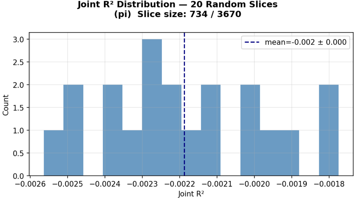
Figure 6: Distribution of Joint R^2 across 20 random slices, \pi null experiment. All 20 draws fall in the range -0.0026 to -0.0018 with \text{std} = 0.000 . The absence of spectral structure is as uniformly distributed as its presence in the positive experiments: no slice finds anything, and the spread across draws is indistinguishable from zero.
