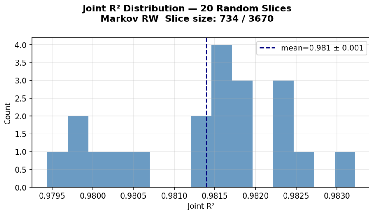
Figure 8: Distribution of Joint R^2 across 20 random slices, nearest-neighbor random walk. All 20 draws fall in the range 0.979–0.984 with \text{std} = 0.001 . The continuously varying asymmetry q across 5,000 distinct environments is linearly readable from any same-size window into the converged parameter vector, with no discreteness artifact inflating the result.
