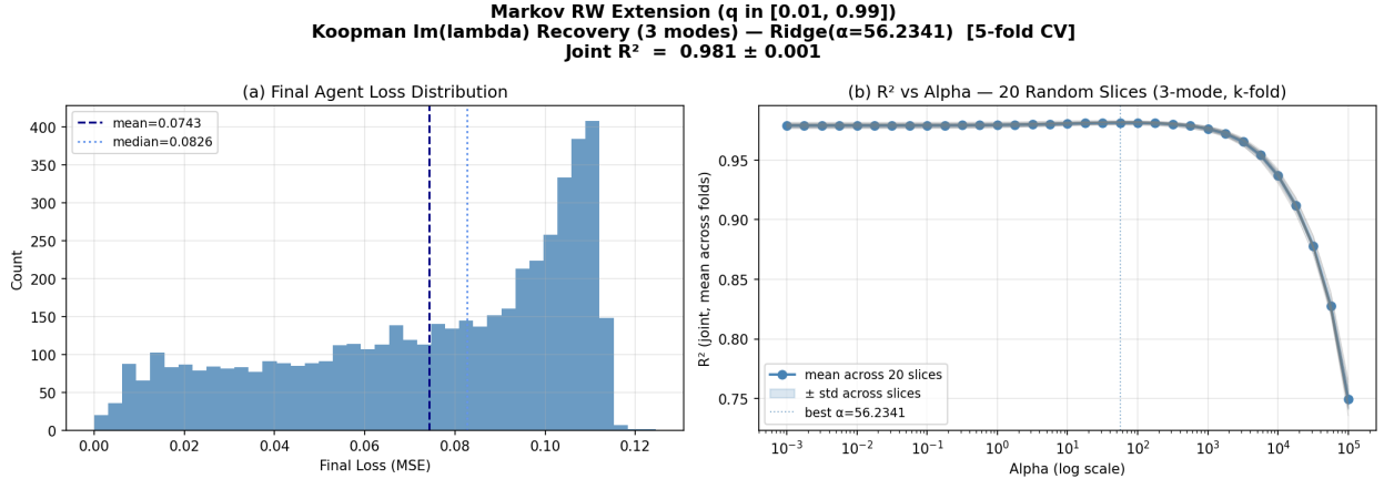
Figure 7: Probe results, nearest-neighbor random walk. (a) Final agent loss distribution. (b) R^2 -vs- \alpha curves for P = 20 random parameter slices (grey) and their mean (blue). The curves are indistinguishable throughout the plateau at R^2 \approx 0.981 , confirming uniform distributed encoding. This is the most demanding test: 5,000 continuously varying environments, a stochastic source, and no discreteness artifact. Joint R^2 = 0.981 \pm 0.001 , range 0.979–0.984. N = 5,000 , T = 200 , N_{\text{modes}} = 3 , d = 734 from D = 3,670 .
